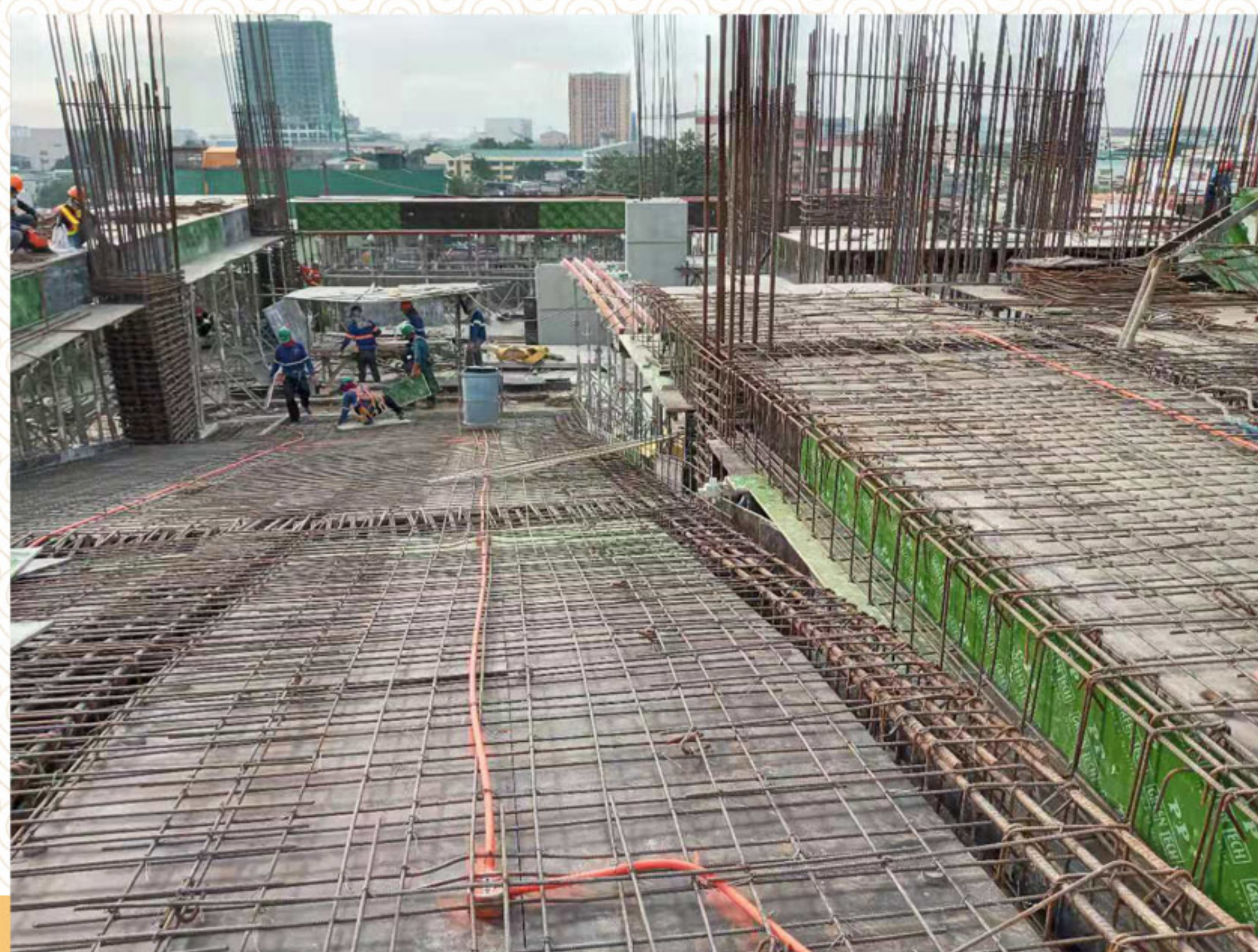
Rebar Works at 5th to 6th Floor Ramp.
