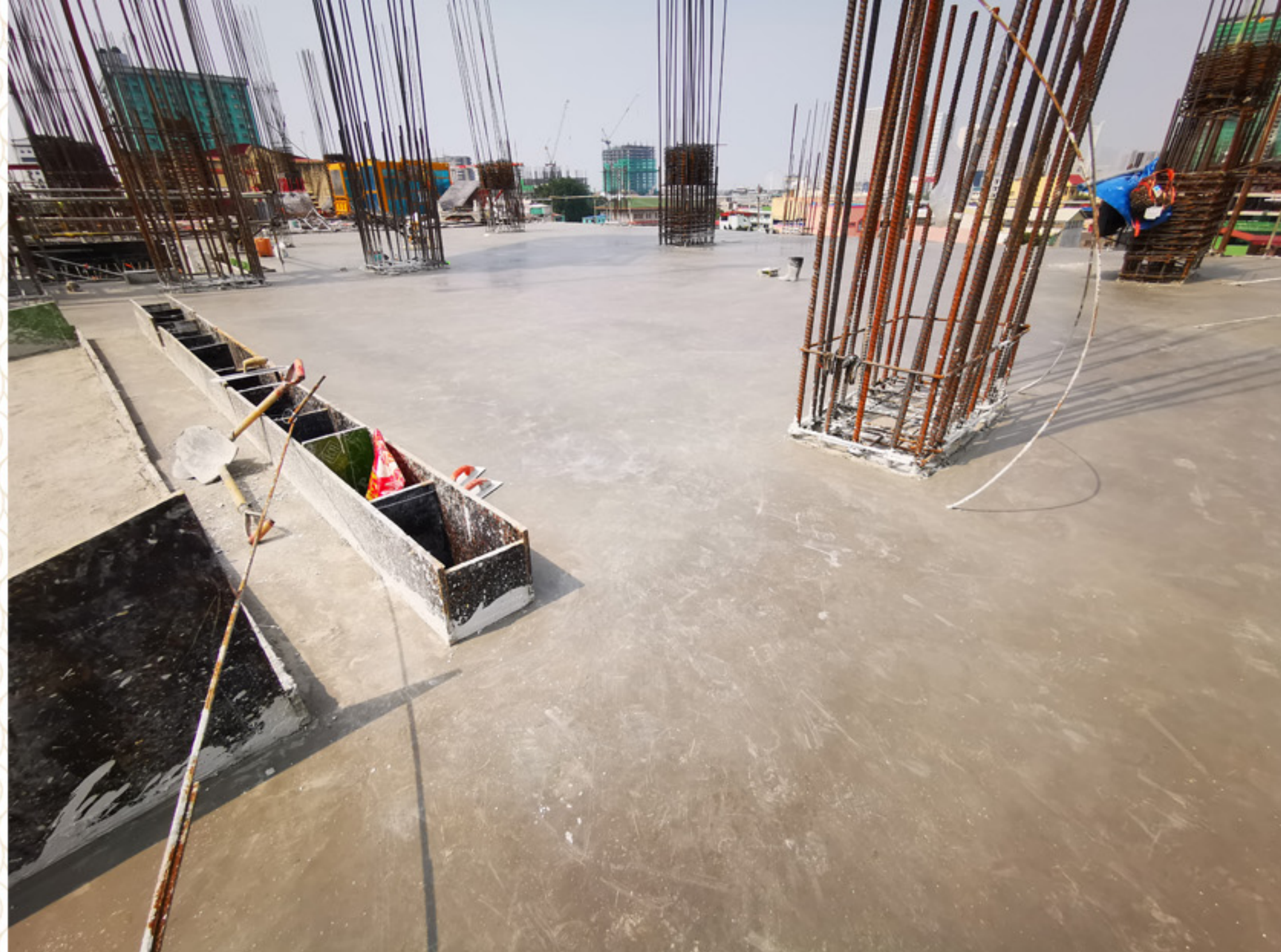
Concreting at 6th Floor, Zone 1. [1區第六樓混凝土樓板]
