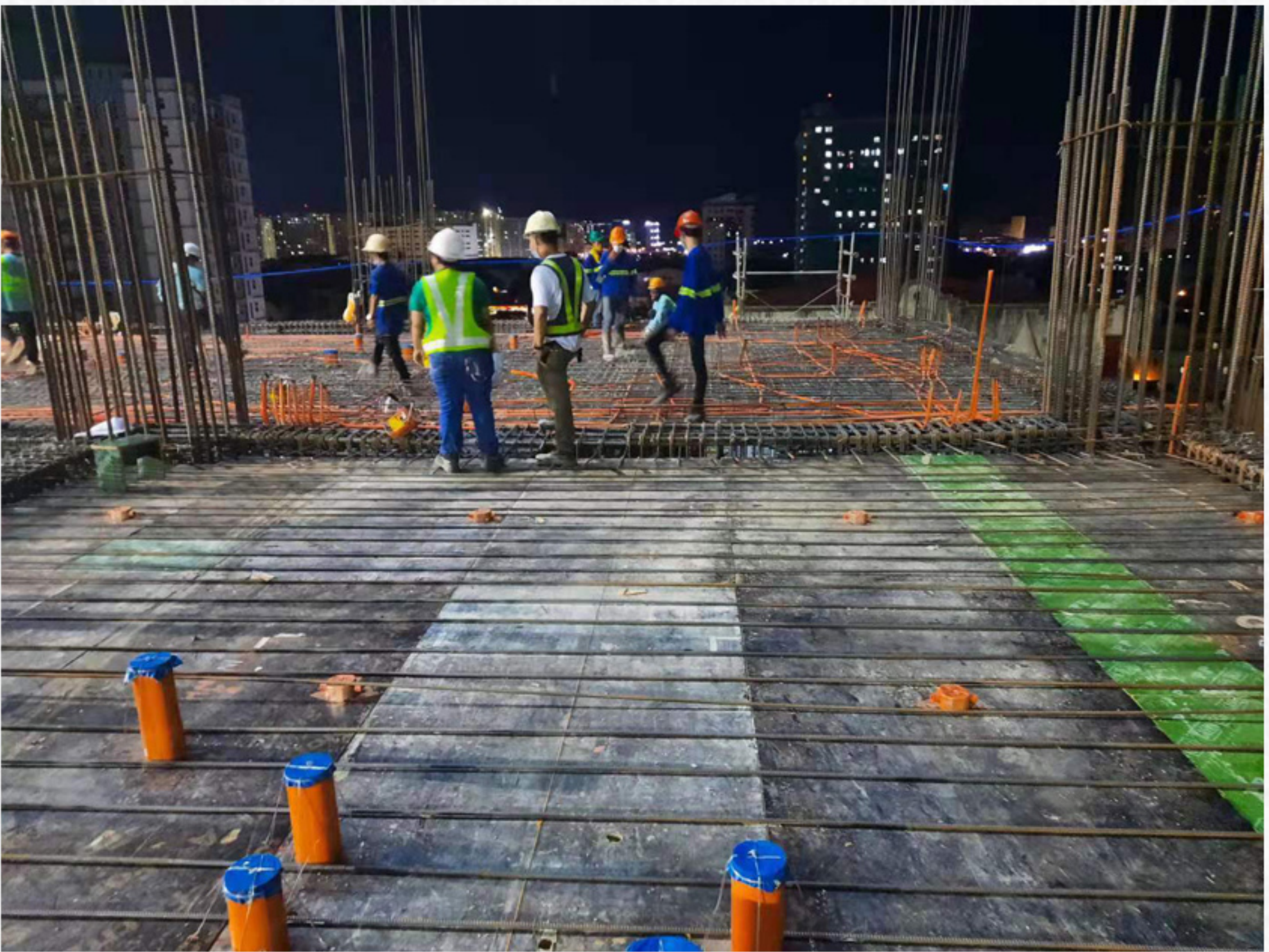
Slab Formworks, Electrical and Plumbing Works at 8th Floor, Zone 2.
